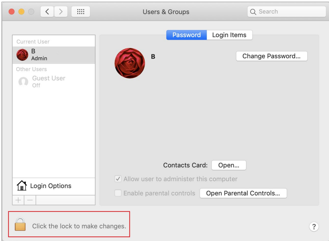
Figure 4. Users & Groups
